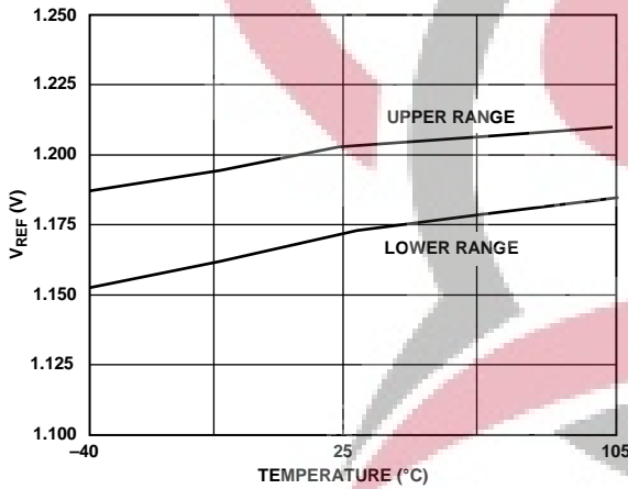
Figure 13. V_{REF} vs. Temperature
