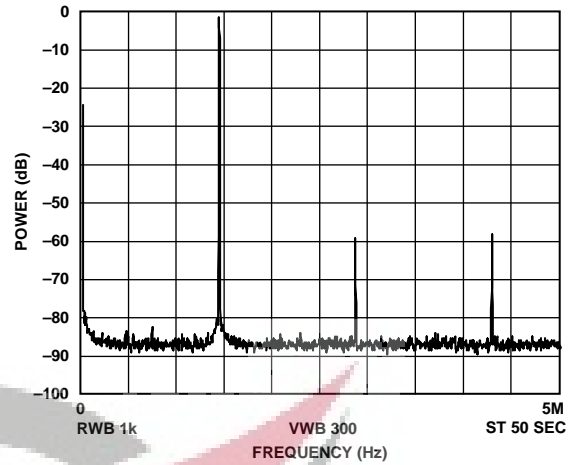
Figure 15. Power vs. Frequency, f_{MCLK} = 10 \text{ MHz} , f_{OUT} = 1.43 \text{ MHz} = f_{MCLK}/7 , Frequency Word = 0x2492492
