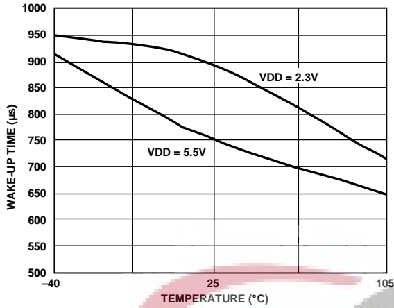
Figure 12. Wake-Up Time vs. Temperature
