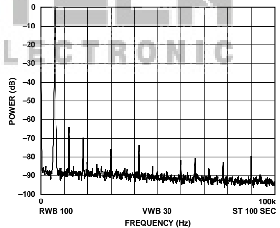
Figure 17. Power vs. Frequency, f_{MCLK} = 25 \text{ MHz} , f_{OUT} = 6 \text{ kHz} , Frequency Word = 0x000FBA9
